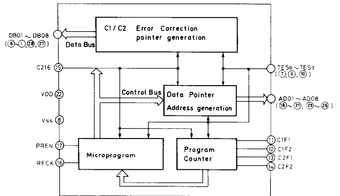
CX7935(Error correction)
