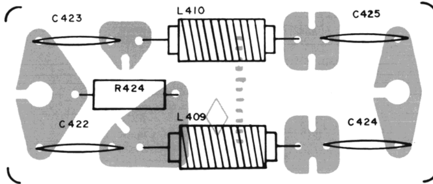
PC-372 AA
